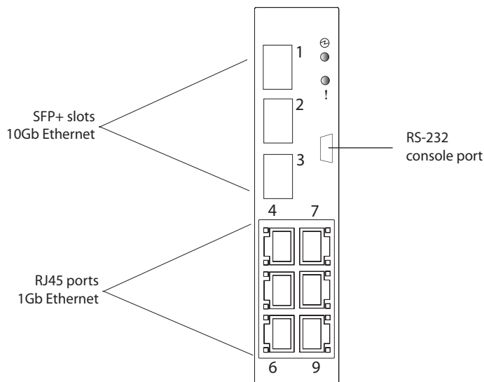
Figure 1 1/10 Uplink Ethernet Switch Module faceplate
