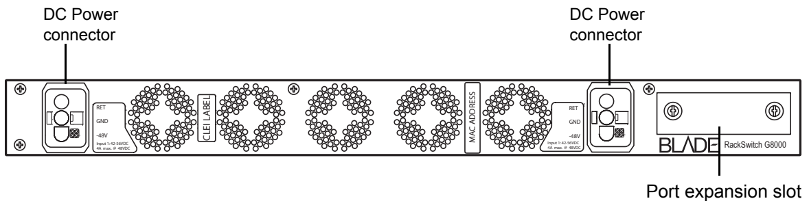
Figure 3 RackSwitch DC G8000 Rear Panel
