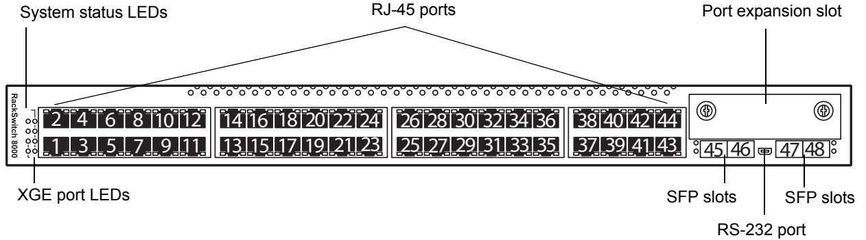
Figure 1 RackSwitch G8000 Front Panel
